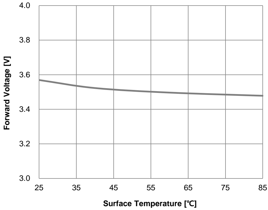
Fig 7. Surface Temperature vs. Forward Voltage, I_F=180\text{mA}
