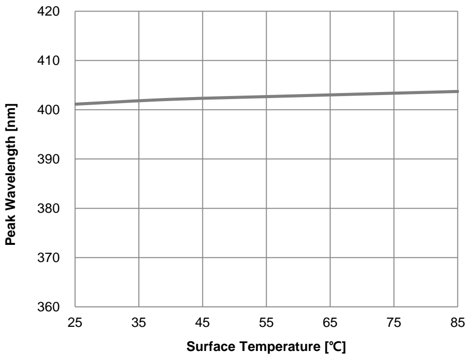
Fig 6. Surface Temperature vs. Peak Wavelength, I_F=180\text{mA}
