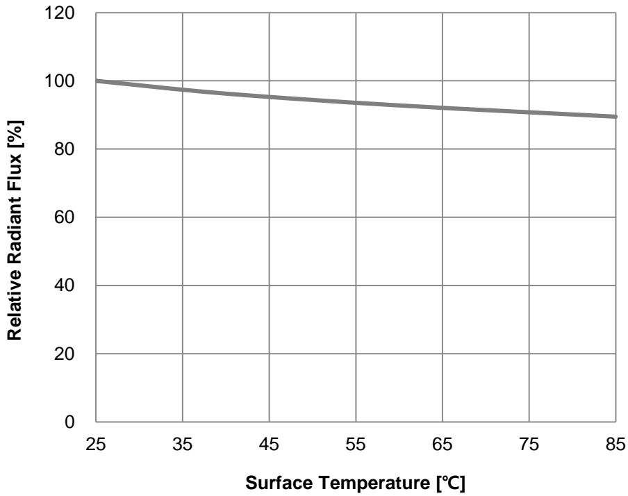
Fig 5. Surface Temperature vs. Relative Radiant Flux, I_F=180\text{mA}
